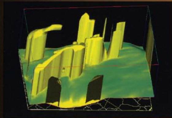
An ozone isosurface plot over the North Carolina UAM simulation domain for the June 1988 air pollution episode.
