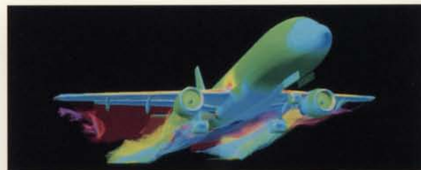
Right, airliner in ground effect. Image shows surface pressure distribution and wakes behind the aircraft.
