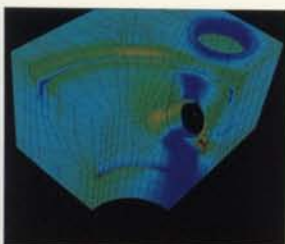
Left, head of a pressure vessel. Colors signify stresses due to pressure and preload.
