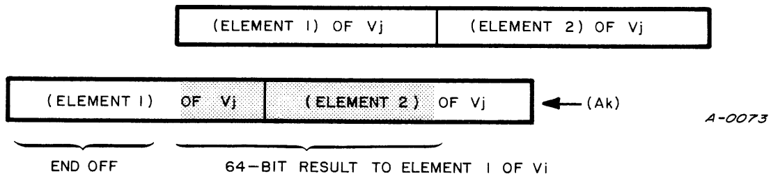
Figure 6-8. Vector left double shift, second element, VL greater than 2
