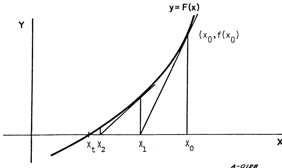
Figure 4-9. Newton's method
