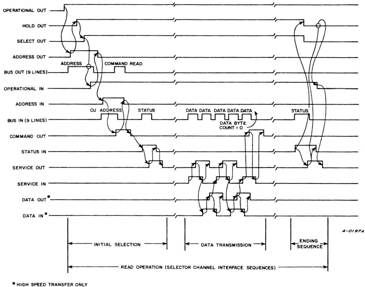
Figure 7-13. Channel read sequence
