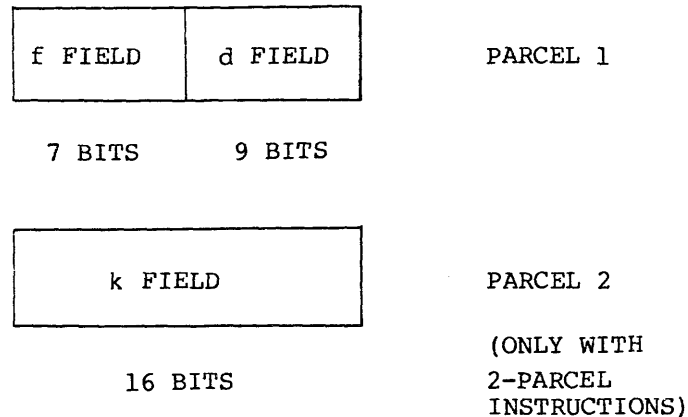
Figure 3-2. Instruction format
