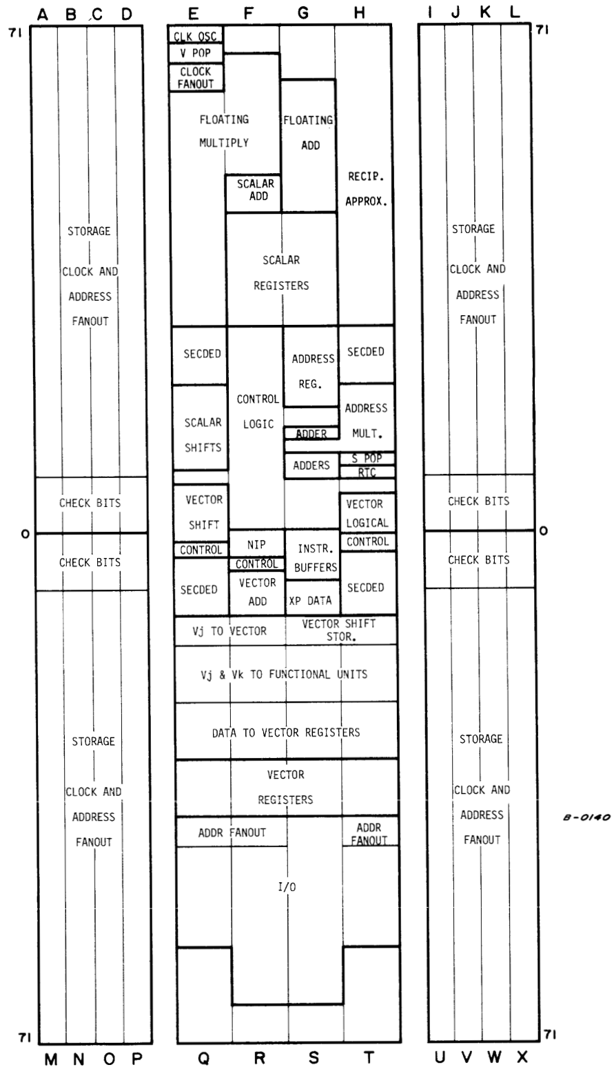
Figure B-2. General chassis layout
