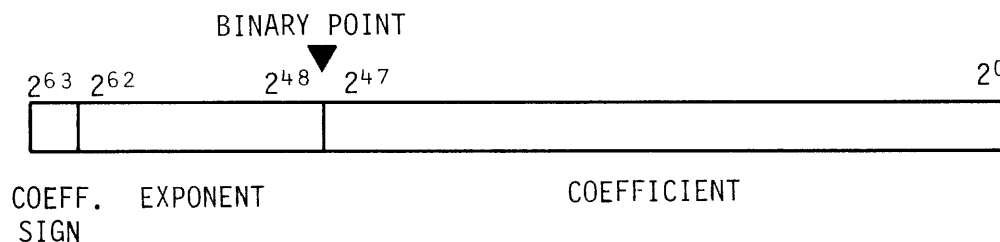
Figure 4-5. Floating-point data formats
